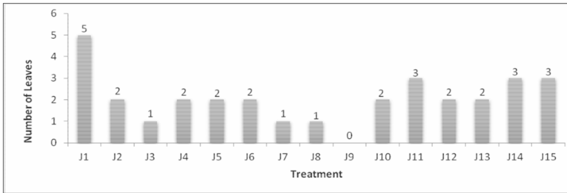
Fig. 8 : Number of Leaves of Batik Bamboo
