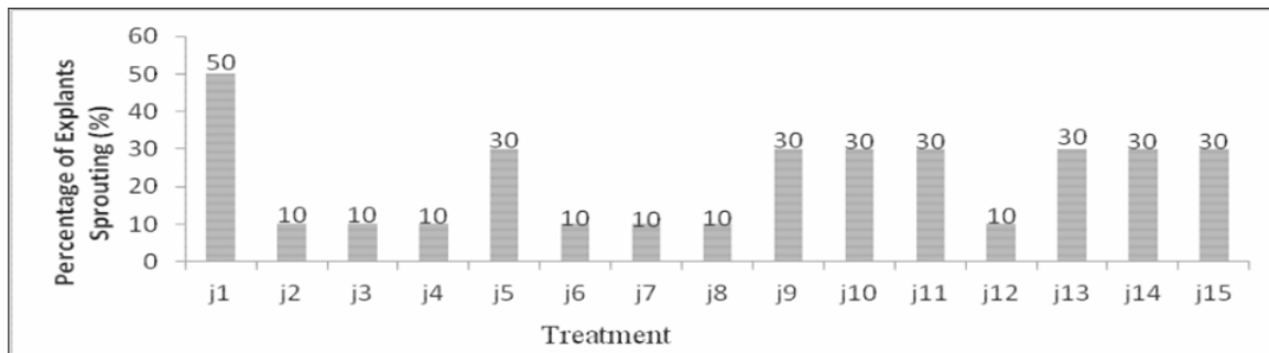
Fig. 4 : Average Percentage of Batik Bamboo Explants Sprouting
