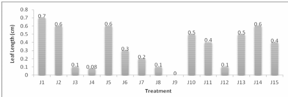
Fig. 9 : Average Length of Batik Bamboo Leaves
