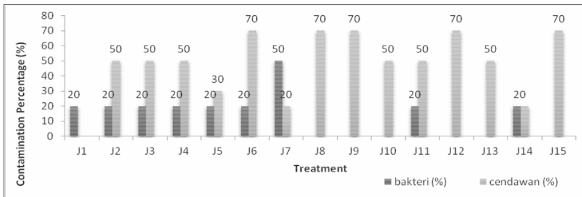
Fig. 10 : The average percentage of Batik Bamboo Contamination
