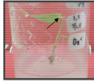
Fig. 7 : Leaves formed after the 8 th week
