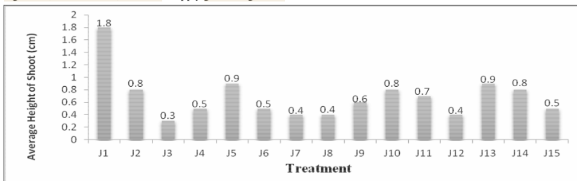
Fig. 6 : Average Height of Shoots of Batik Bamboo
